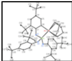
Fig. 1. The molecular structure of the title compound showing the atom-labelling scheme. Hydrogen atoms and the disordered toluene are omitted for clarity. Displacement ellipsoids are drawn at the 30% probability level.
